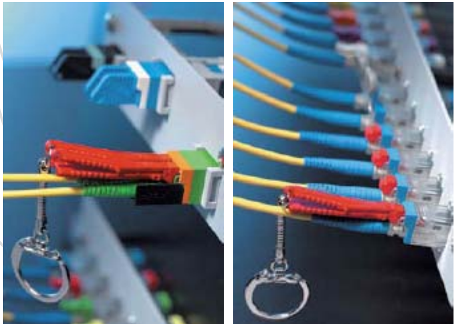
A new security solution for the E-2000™ fibre optic connector. Patch Guard locks the connection which can then only be locked with a special key.
